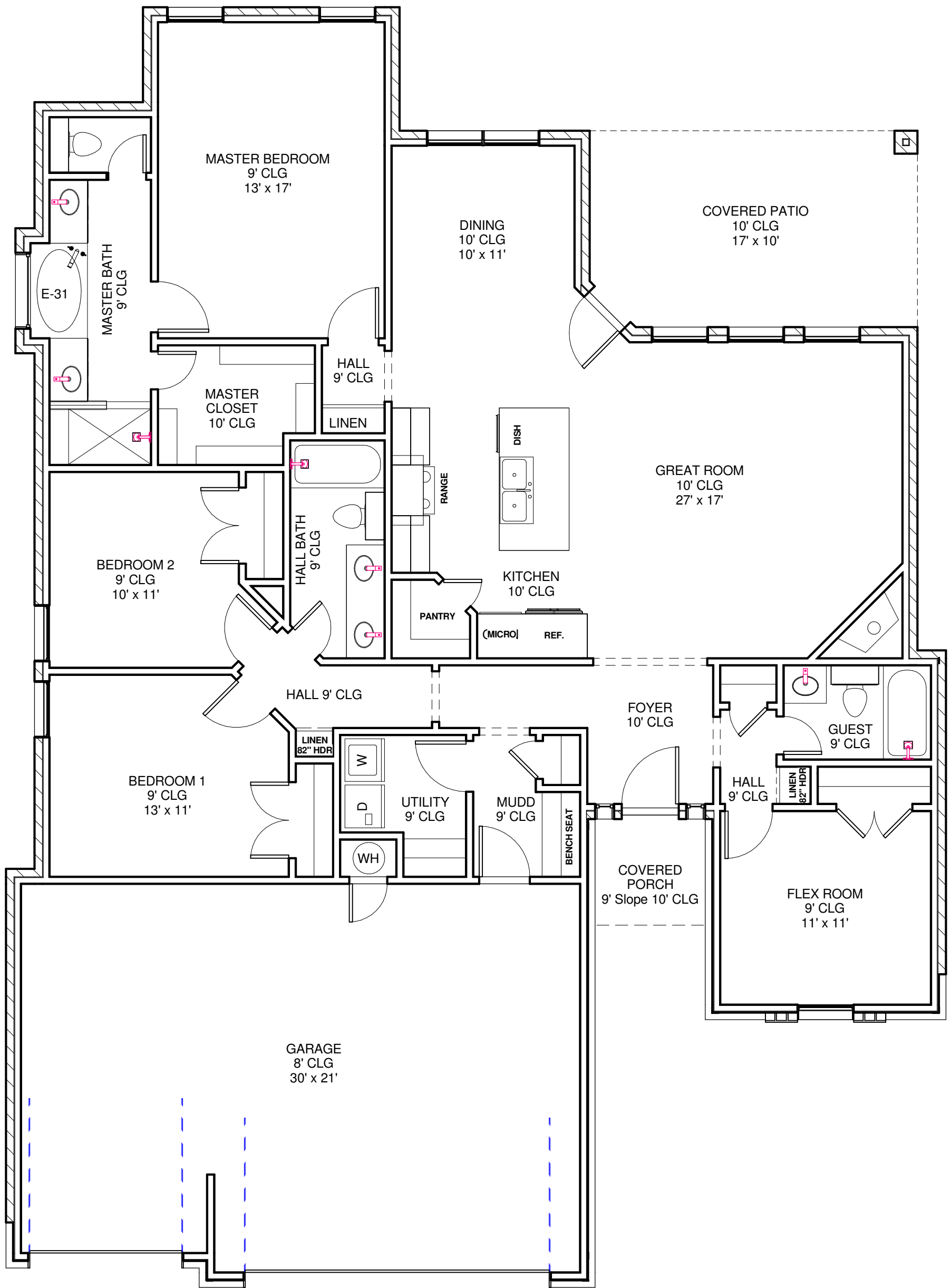
1 Floor Plan - Preliminary Design 1 3/16" = 1'-0"
